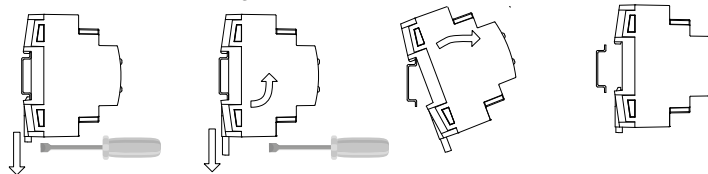
Removing ALLinBOX 1612 v2 from DIN rail:
